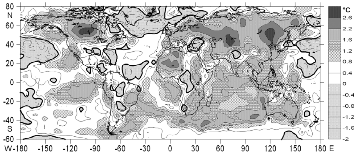
Fig. 2. Linear surface air temperature trends 1951-2000 in °C within the 80°N-60°S zone in a 5° grid resolution, contour lines at 0.4 °C intervals. Data source: Jones, 2007; analysis: Schönwiese (2003, updated). The heavy lines encircle areas where a temperature decrease is observed (within these areas dashed contour lines).
