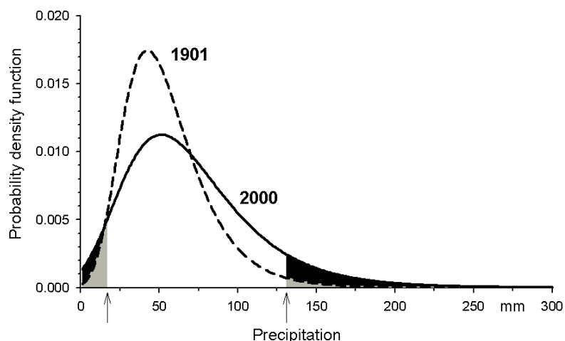
Fig. 9. Probability density function (PDF) change 1901-2000 of the January precipitation at station Eppenrod, Germany (50.4° N, 8.0° E), where the arrows indicate the (lower) 5th and the 95th (upper 5th) percentiles which amount to 17 mm or 131 mm, respectively, at this station. The related extreme value occurrence probabilities (indicated by grey or black shading, respectively) have increased for both extreme low and extreme high precipitation (for more explanation see text; from Schönwiese, Trömel, and Janoschitz, 2007).
