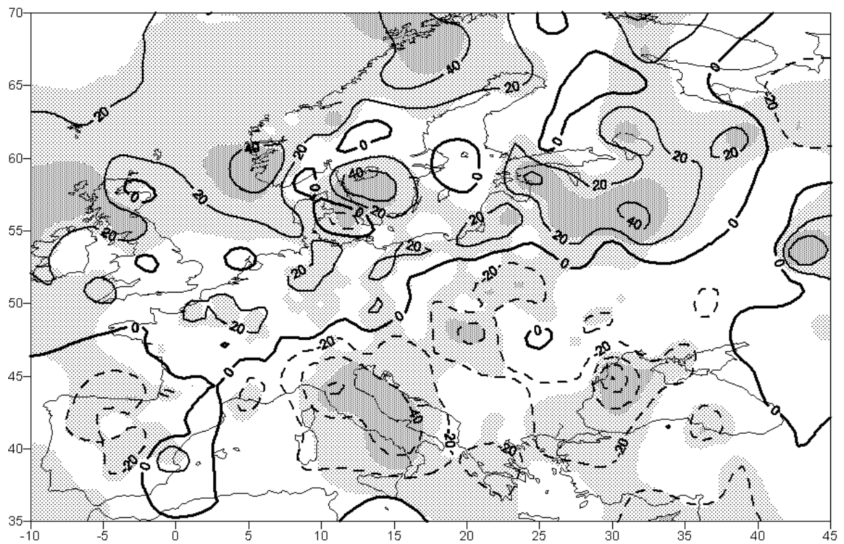
Fig. 8. Linear precipitation trends 1951-2000, European pattern, in absolute (mm, upper plot) and percent (lower plot) values, winter (December of previous year, January, and February (from Beck et al., 2007, based on Schönwiese and Janoschitz, 2007).
