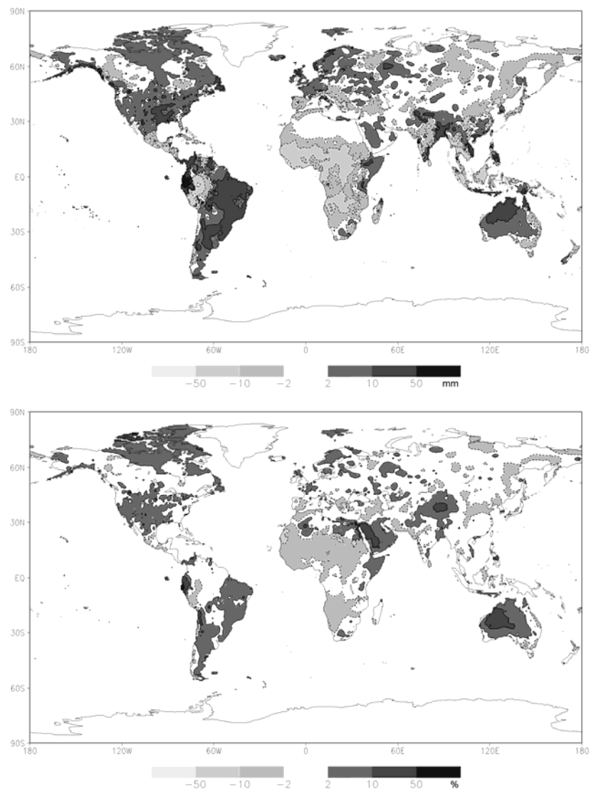
Fig. 6. Linear annual precipitation trends 1951-2000 in mm (upper plot) and percent (lower plot) per month, global patterns, 5° grid resolution (from Beck et al., 2007, modified). White areas neglected due to a small data base (Greenland, Antarctica, and a small region in northeast Africa). Dashed contour lines indicate a decrease.
