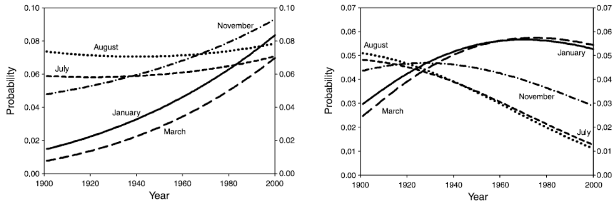
Fig. 10. Change 1901-2000 of the probability of occurring extremes (a, left) above the 95 th percentile and (b, right) below the 5 th percentile of precipitation in selected months at station Eppenrod, Germany (from Trömel and Schönwiese, 2007).
