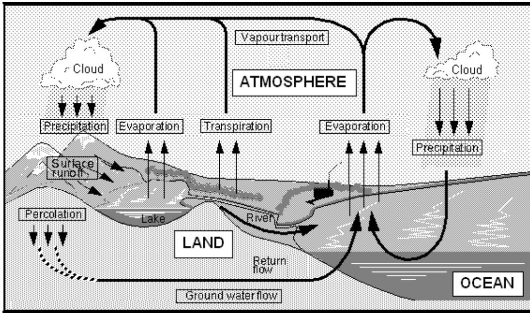
Fig. 3. Scheme of the global water cycle (from CHIAS, 2007, modified). Quantitative description see Table 1.
