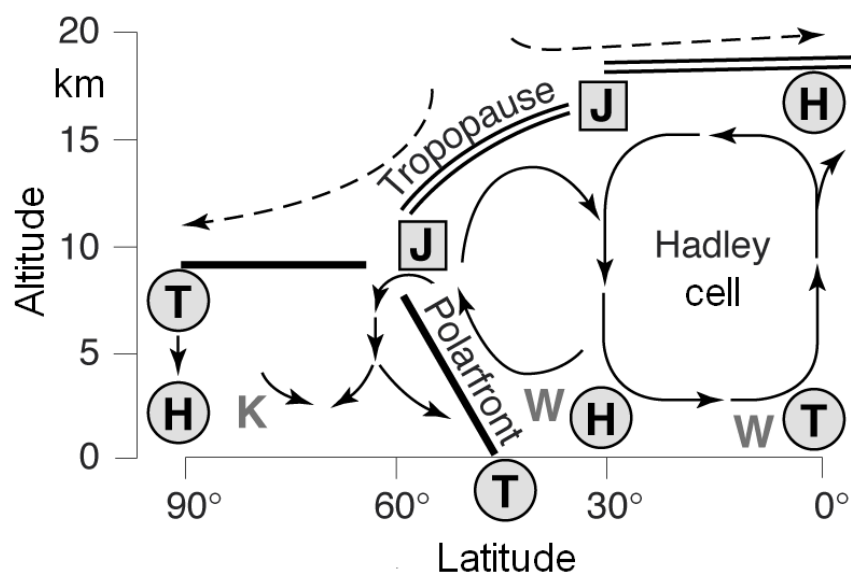
Fig. 4. Cross section of the atmospheric circulation, schematic, troposphere, one hemisphere (from Schönwiese, 2003, modified). Note that, in general, uplift (low pressure near surface, T) leads to cloud formation and precipitation whereas subsidence (high pressure near surface, H) to dryness. W means warm, K cold air masses; J = jet stream.
