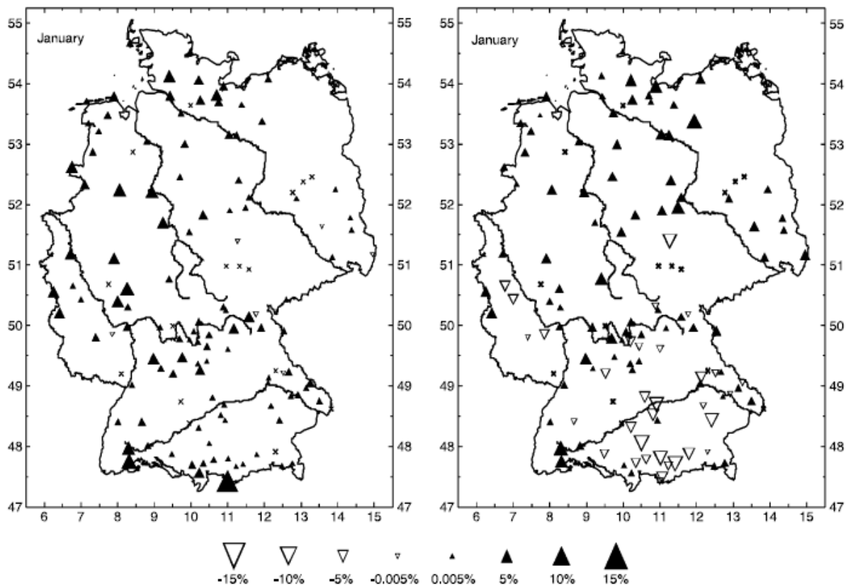
Fig. 11. Changes 1901-2000 of the probability of extreme January precipitation occurring above the 95 th , left, or below the 5 th percentile, right, at 132 stations in Germany. Upward black triangles indicate an increase and white downward triangles a decrease of this probability. The caption denotes the related magnitude (from Trömel and Schönwiese, 2007).
