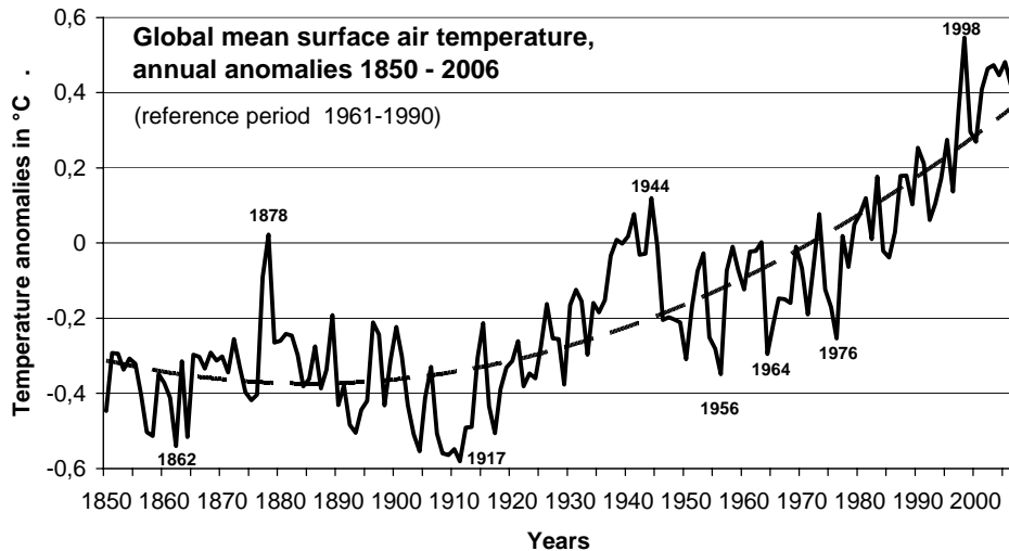
Fig. 1. Annual anomalies 1850-2006 of the global mean surface air temperature (from Jones, 2007). The dashed line indicates the polynomial trend. The linear trend 1901-2000 amounts to 0.7 °C.
