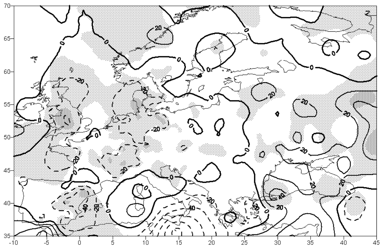
Fig. 7. Linear precipitation trends 1951-2000, European pattern, in absolute (mm, upper plot) and percent (lower plot) values, summer (June, July, and August) data (from Beck et al., 2007, based on Schönwiese and Janoschitz, 2007).
