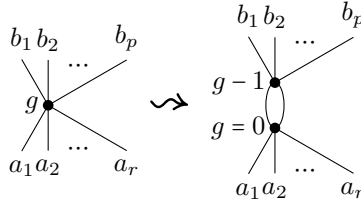
FIGURE 8. Splitting positive genus
