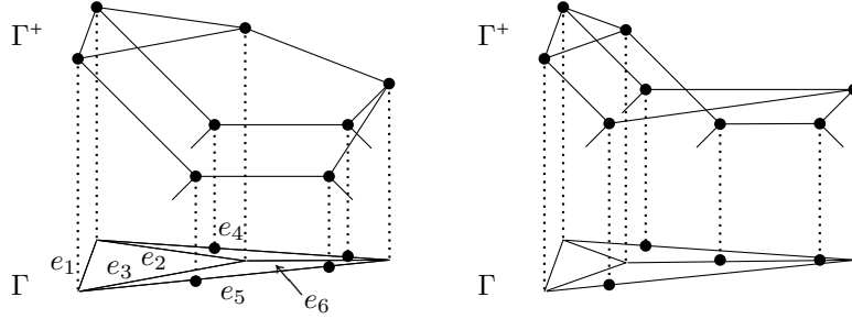
FIGURE 4. Realizable configurations of maximal dimension on K_4 : 3-cycles on top level, edges with two points
