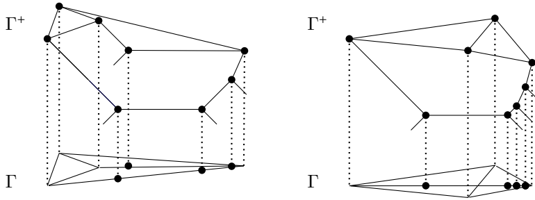
FIGURE 5. Realizable configurations of maximal dimension on K_4 : 3-cycles on top level, more than two points on some edge
