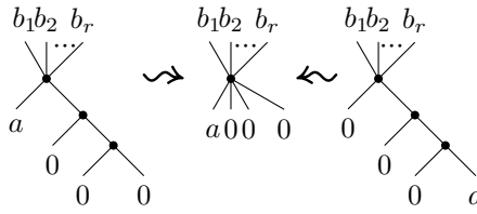
FIGURE 9. Rearranging trees of marked points
