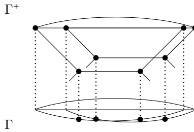
FIGURE 6. Realizable configurations of maximal dimension on K_4 : 4-cycle on top level
