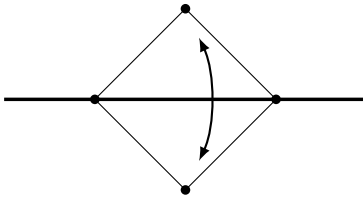
FIGURE 7. The simplices over the dumbbell graph
