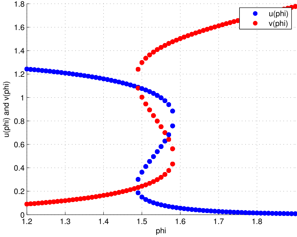
Figure 3.1: A triple solution.
